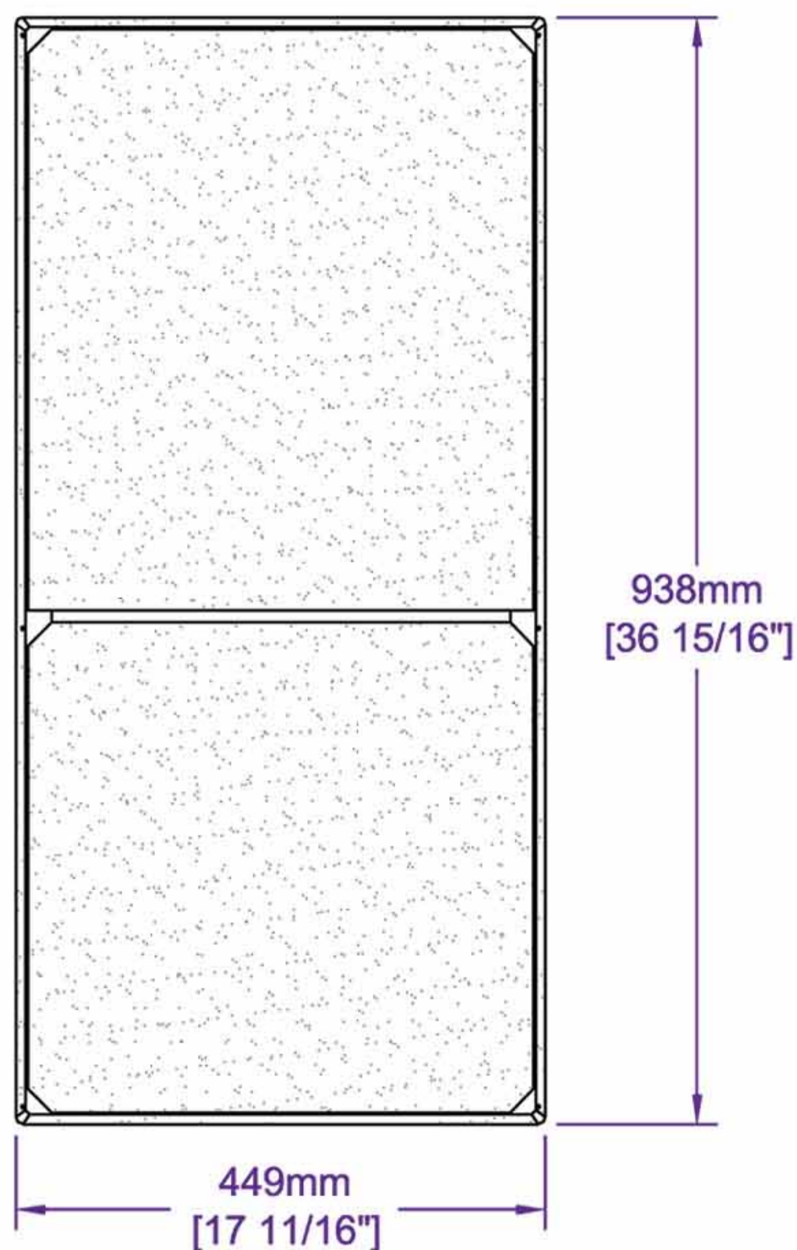
Back showing stainless steel frame
